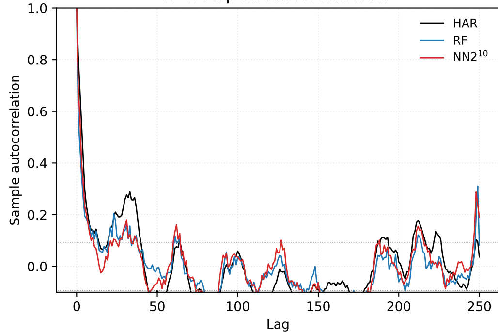
h=1-step-ahead forecast ACF
