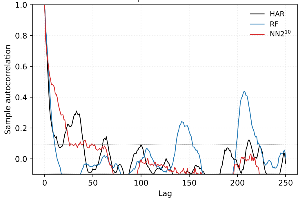
h=22-step-ahead forecast ACF
