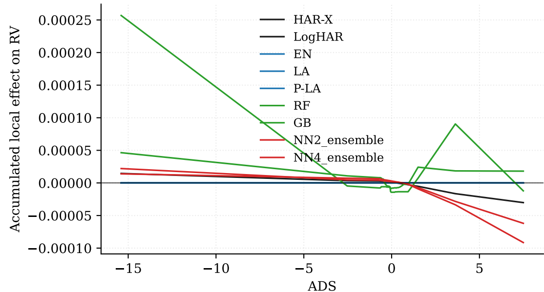
ALE for ADS on AAPL
