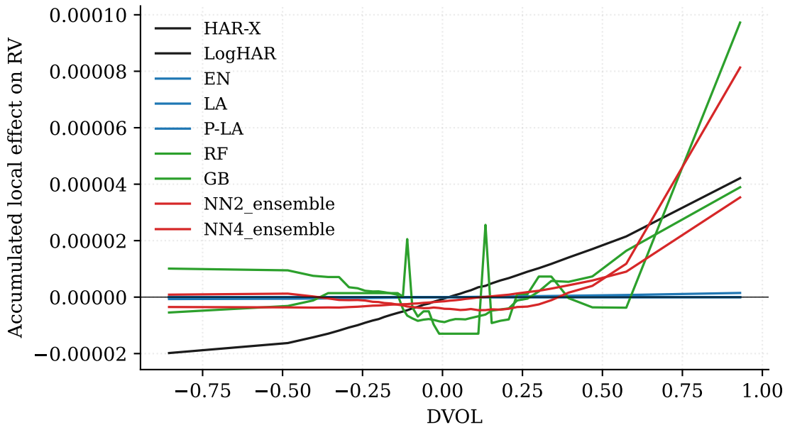
ALE for DVOL on AAPL
