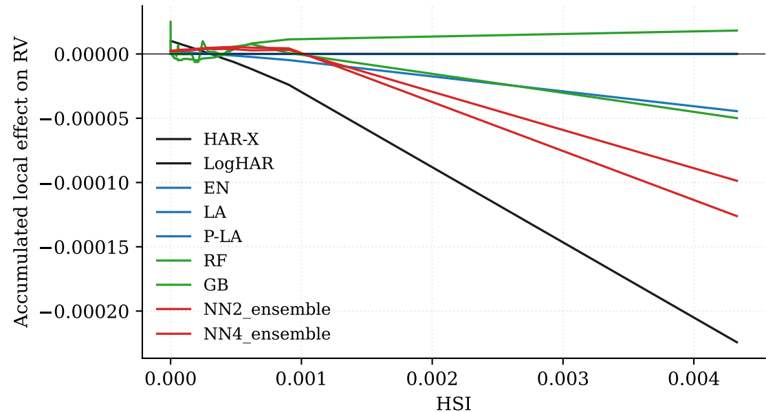
ALE for HSI on AAPL
