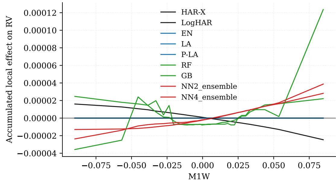
ALE for M1W on AAPL
