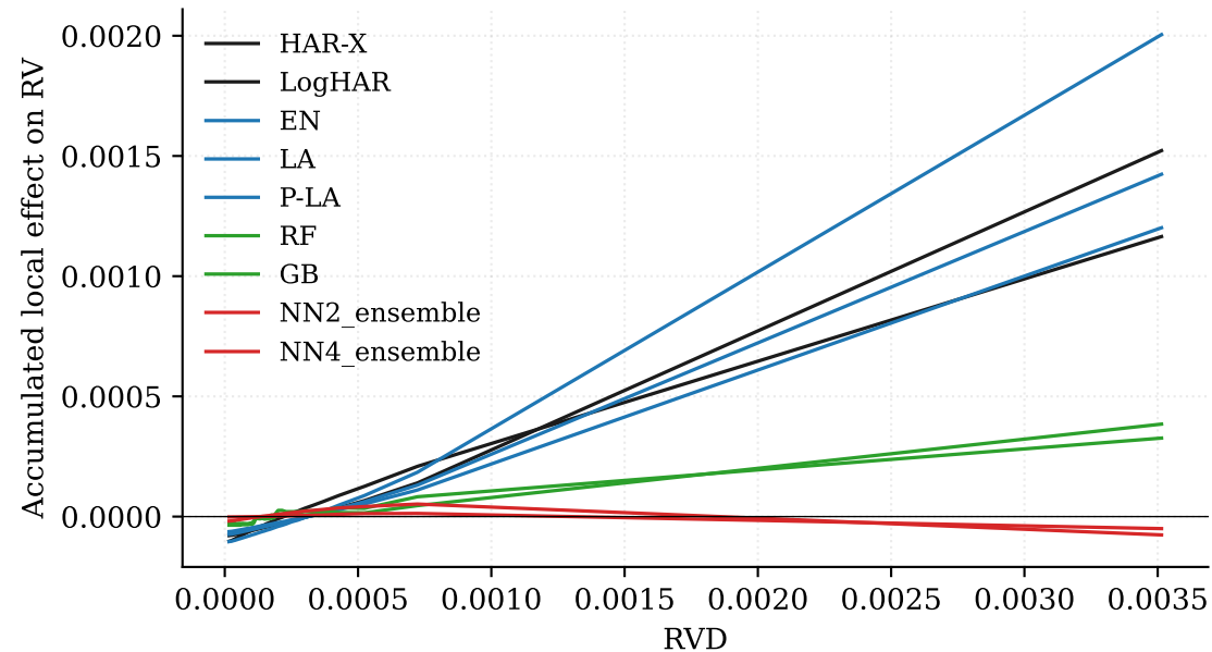
ALE for RVD on AAPL
