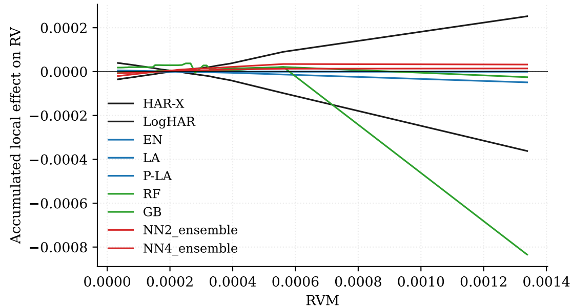
ALE for RVM on AAPL
