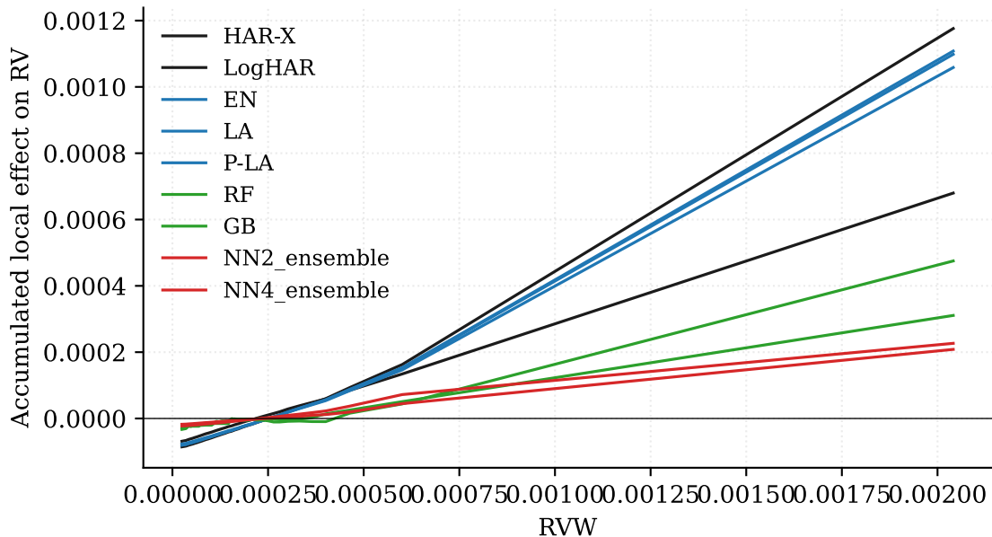
ALE for RVW on AAPL
