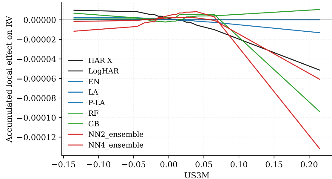
ALE for US3M on AAPL
