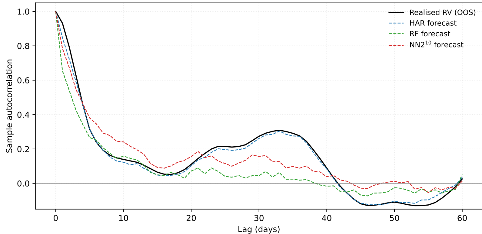
Out-of-sample ACF: realised vs forecast (AAPL, h=5)
