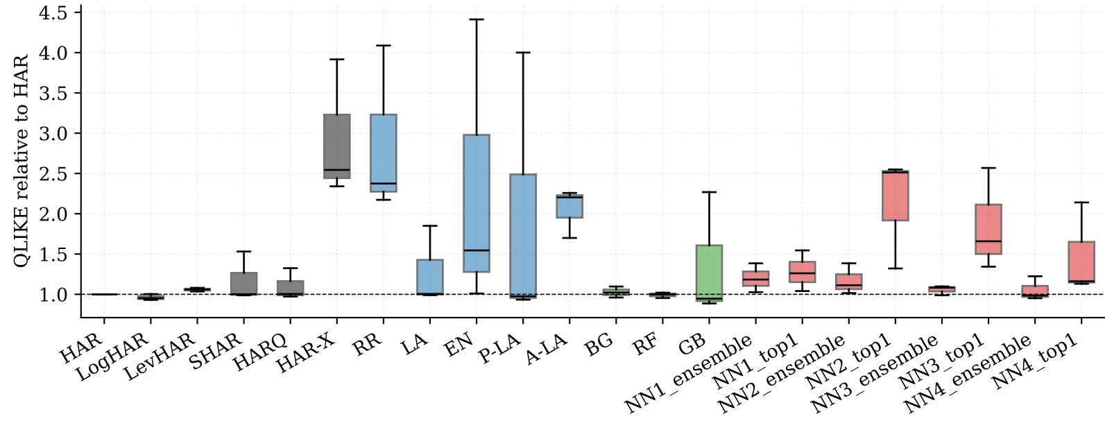
QLIKE ratio to HAR, h=1
