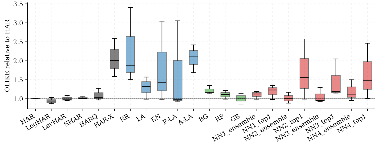
QLIKE ratio to HAR, h=5
