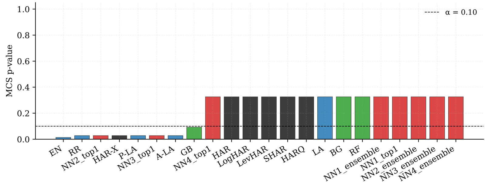
MCS — AMZN, h=1
