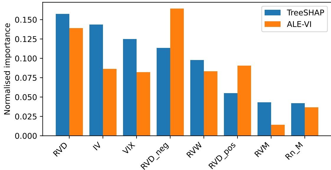
RF — AAPL h=1: TreeSHAP vs ALE
