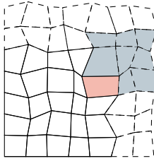
Fig. 11.3. Illustration of mesh partition. Ghost cells are drawn with dashed lines. The size of ghost layer is determined by the number of cells need in the time stepping computation.
