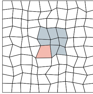
Fig. 11.1. Logically rectangular mesh displayed in full. The index of a stencil (colored cells) is the same as the index of the red cell.
