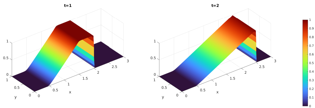
Figure 3: The reconstructed solution on the 180 \times 60 rectangular mesh at times 1.0 and 2.0. (The rarefaction and shock meet at time 2.0.)
