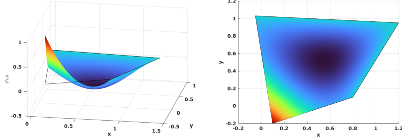
Figure 1.5: Vertex nodal basis function \varphi_{v,0}^{(2)} in \mathcal{DS}_2 .
