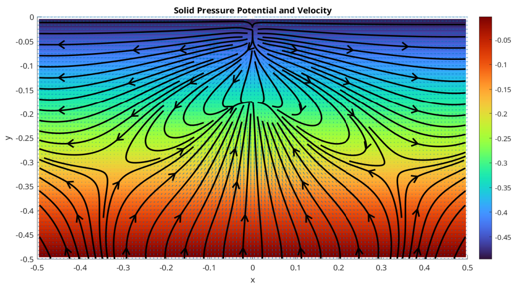
Figure 1.7: Solid pressure potential and velocity.
