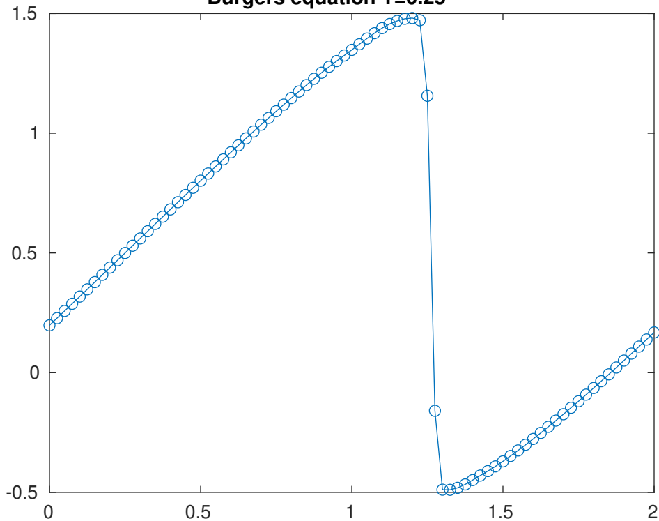
Burgers equation T=0.25
