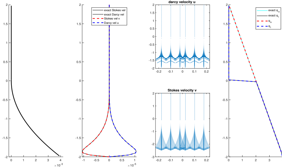
Figure 3: Quadratic porosity compaction column test.
