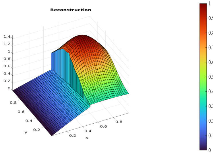
Figure 3.22: The reconstructed solution on the 20 \times 20 randomly distorted logically rectangular mesh.
