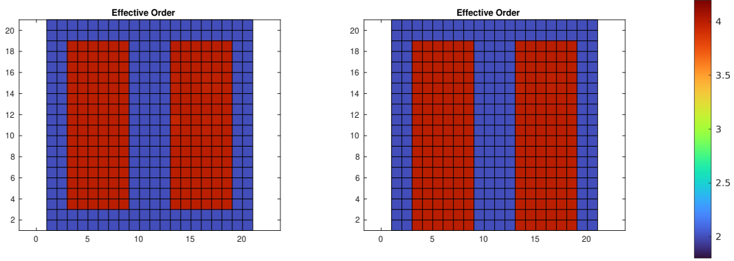
Figure 6: Effective reconstruction order with and without some additional fifth-order stencils on one side of the boundary y = 0 .
