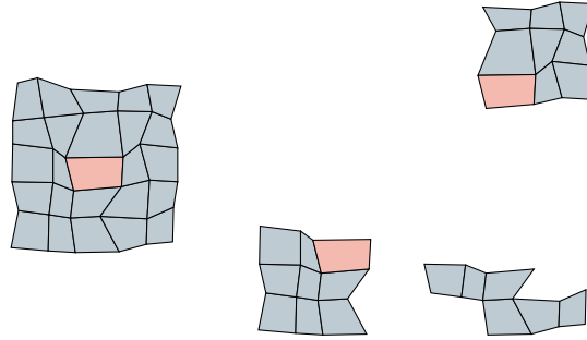
Figure 3: An example of a standard (5,3) stencils combination on a logically rectangular quadrilateral mesh.
