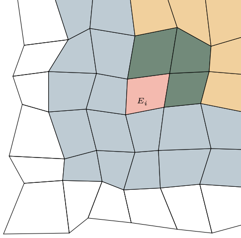
Figure 4: An illustration of three different cells sharing the same fifth order stencil.
