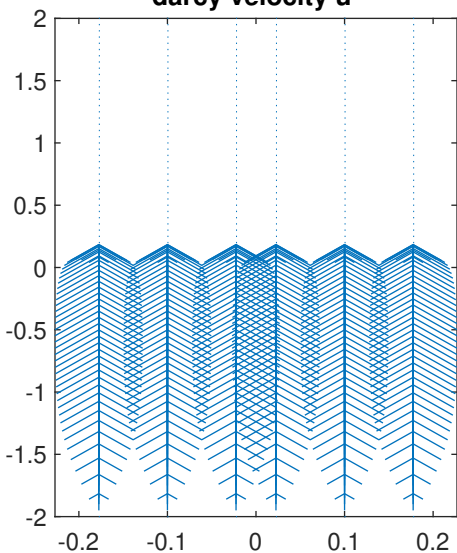
darcy velocity u
