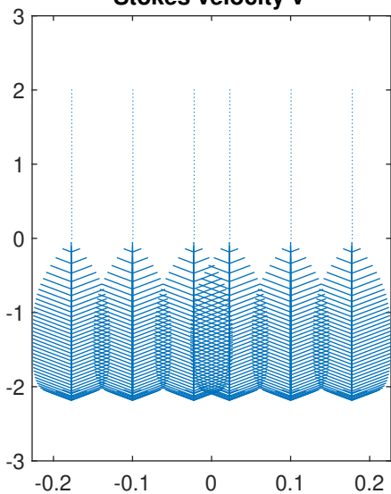
Stokes velocity v
