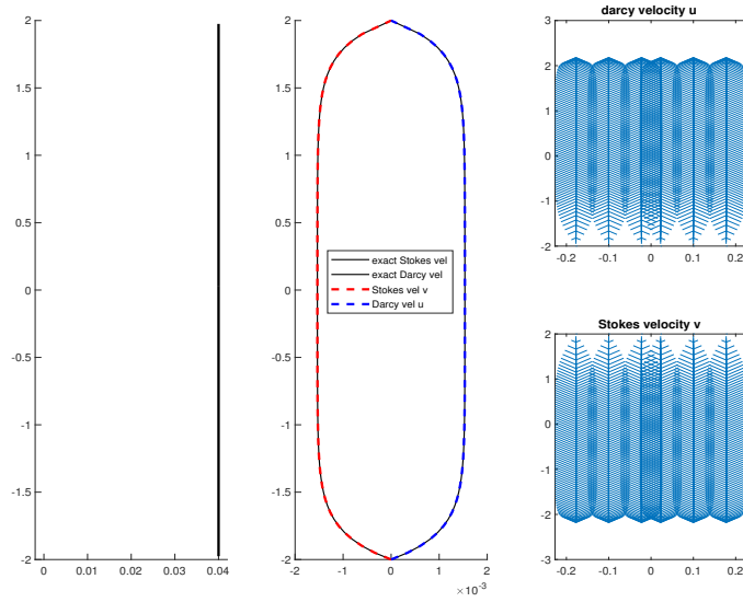
Figure 1.11: Constant porosity compaction column test.
