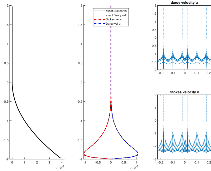
Figure 1.13: Quadratic porosity compaction column test.
