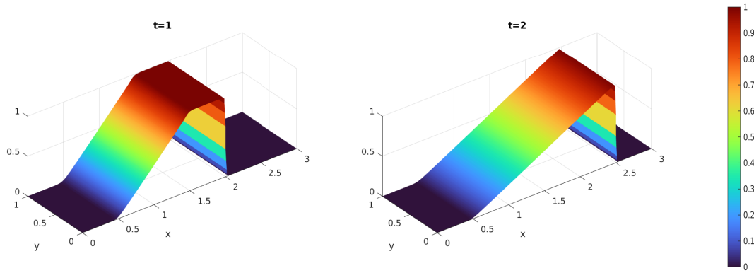
Figure 5: The reconstructed solution on the 180 \times 60 rectangular mesh at times 1.0 and 2.0. (The rarefaction and shock meet at time 2.0.)
