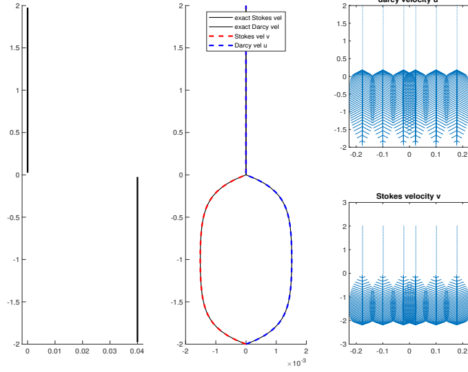
Figure 1.2: Piecewise constant porosity compaction column test.
