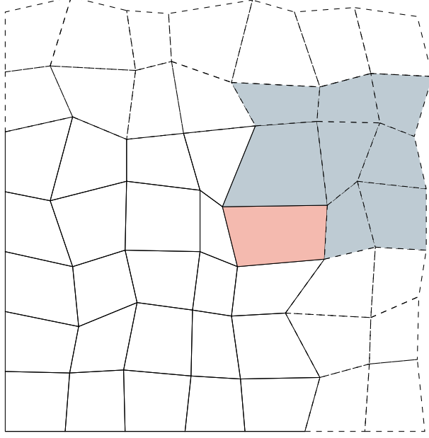
Figure 1.2: An exhibition of ghost region in parallel implementation of ML-WENO scheme.
