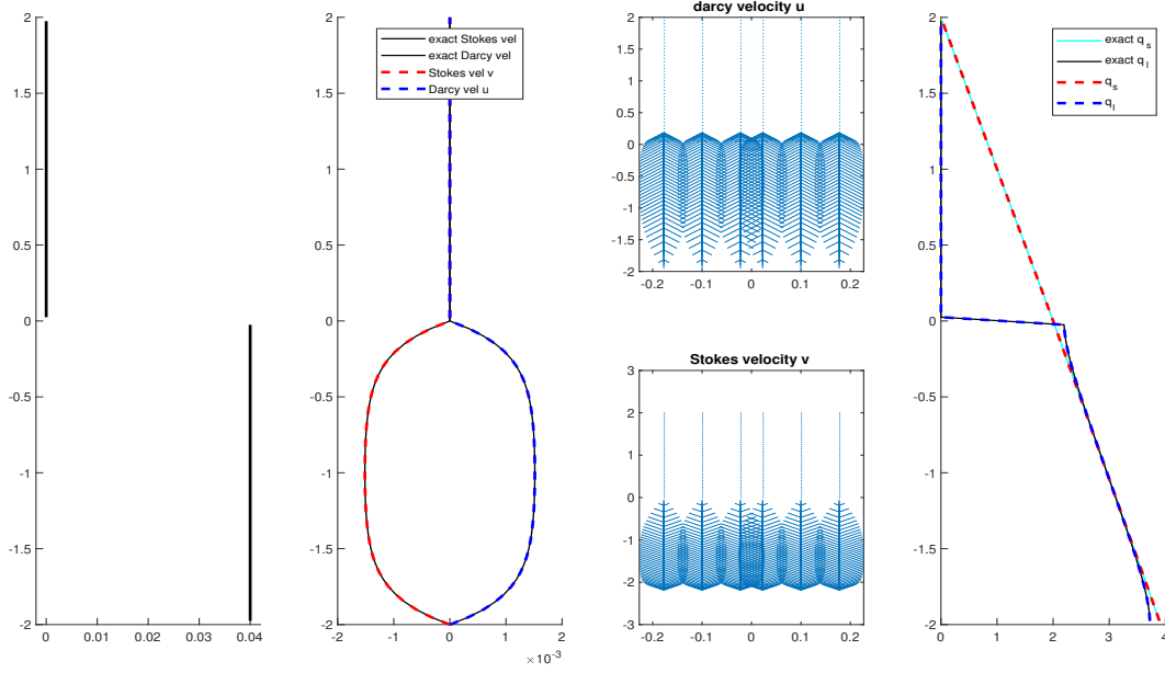
Figure 3.12: Discontinuous porosity (3.158) with \phi_0 = 0.04 . Shown are the porosity \phi , scalar velocities u and v along with closed form solution, velocity vectors \mathbf{v}_s and \phi \mathbf{v}_r reconstructed on the edge quadrature points, q_l and q_s together.
