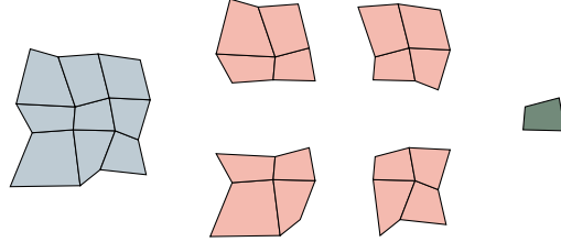
Figure 2.1: An example of (3,2,1) multi-level stencils combination on logically rectangular quadrilateral mesh.
