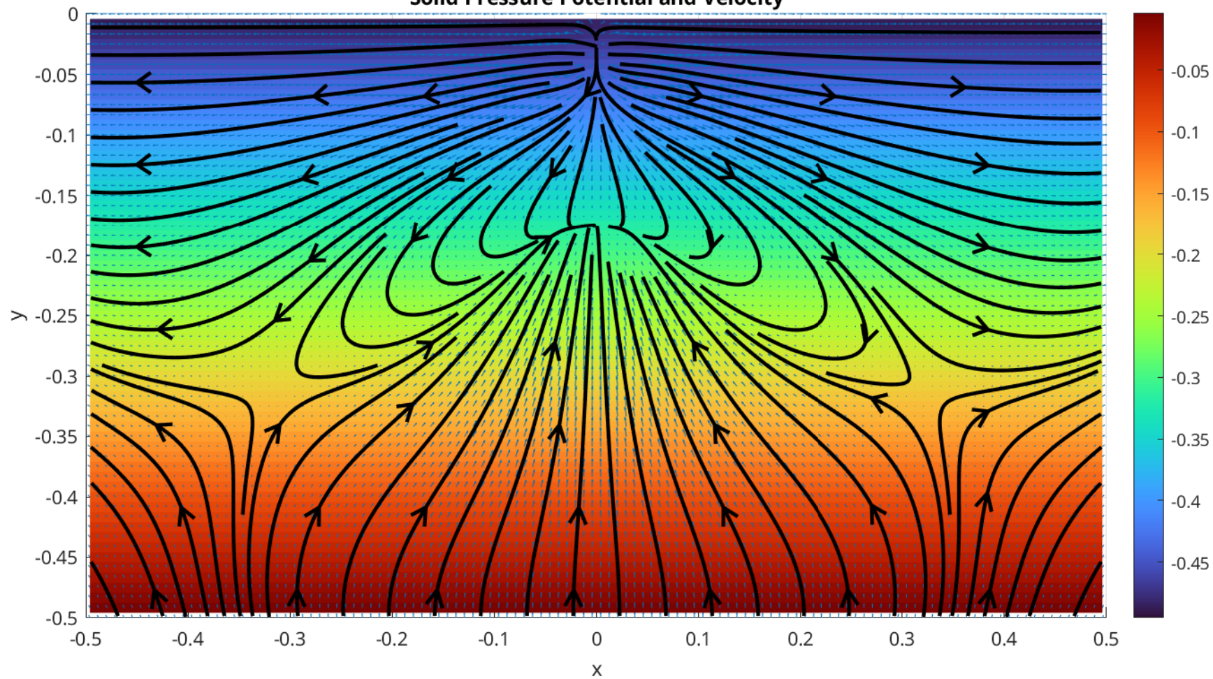
Solid Pressure Potential and Velocity
