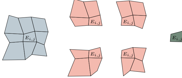
Figure 1.7: An example of (3,2,1) multi-level stencils combination on logically rectangular quadrilateral mesh.
