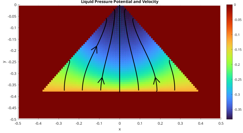
Figure 1.5: Liquid pressure potential and velocity.
