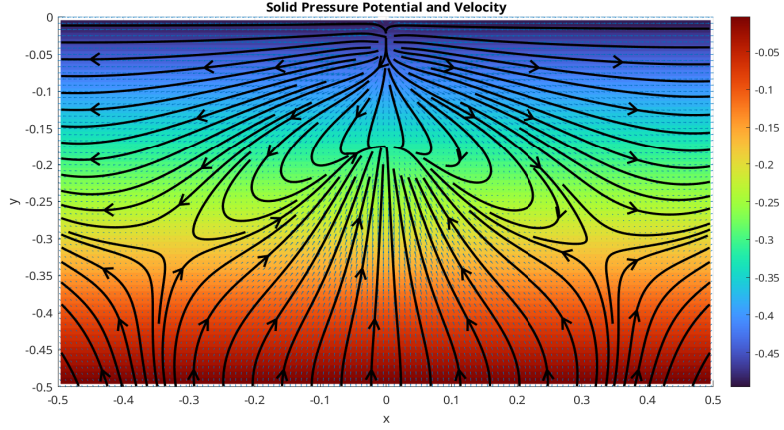
Figure 1.6: Solid pressure potential and velocity.
