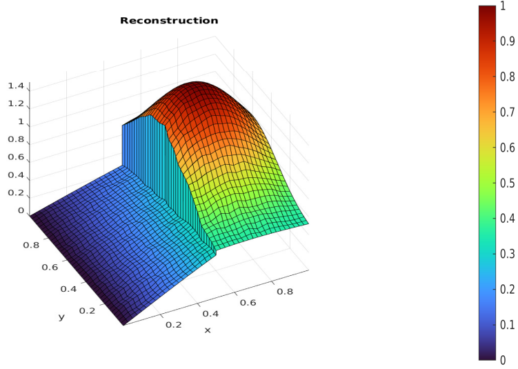
Figure 4: The reconstructed solution on the 20 \times 20 randomly distorted logically rectangular mesh.
