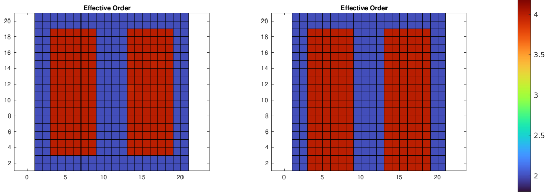
Figure 5: Effective reconstruction order with and without some additional fifth-order stencils on one side of the boundary y = 0 .
