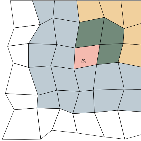
Figure 3: An illustration of three different cells sharing the same fifth order stencil.
