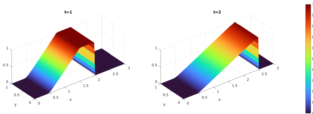
Figure 6: The reconstructed solution on the 180 \times 60 rectangular mesh at times 1.0 and 2.0. (The rarefaction and shock meet at time 2.0.)
