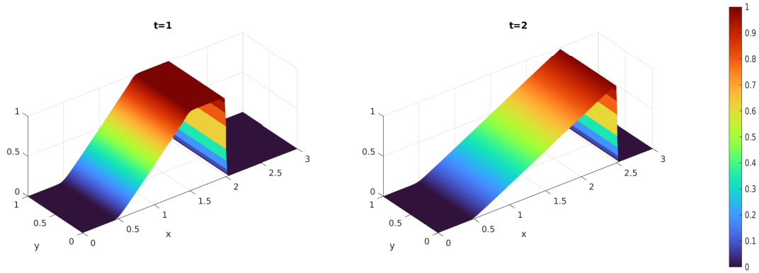
Figure 3: The reconstructed solution on the 180 \times 60 rectangular mesh at times 1.0 and 2.0. (The rarefaction and shock meet at time 2.0.)
