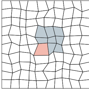
Fig. 9.1. Logically rectangular mesh displayed in full. The index of a stencil (colored cells) is the same as the index of the red cell.
