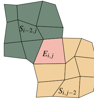
Fig. 9.2. Two sample stencils used by cell E_{i,j} . The index of these two stencils are S_{i-2,j} and S_{i,j-2} . Consistent with the index of bottom left cell.
