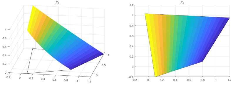
Figure 1.2: Rational function R_0 .
