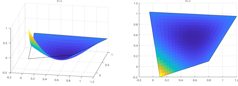
Figure 1.4: Vertex nodal basis function \varphi_{v,0} is \mathcal{DS}_2 .
