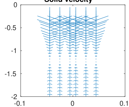
Solid velocity
