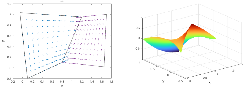
Figure 1.8: “Linear” shape function \boldsymbol{\varphi}_l .
