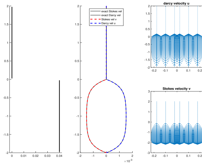
Figure 1.12: Piecewise constant porosity compaction column test.
