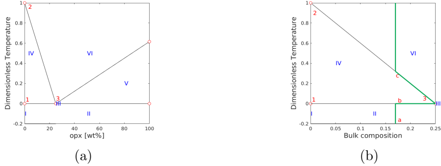
Figure 1.2: Eutectic Phase Diagram. (a) Full phase diagram of olivine-opx system. (b) Phase diagram when composition of opx smaller than eutectic composition.
