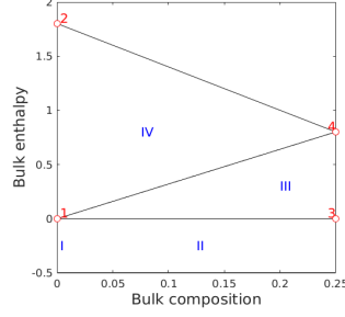
Figure 1.3: Enthalpy-Composition Diagram
