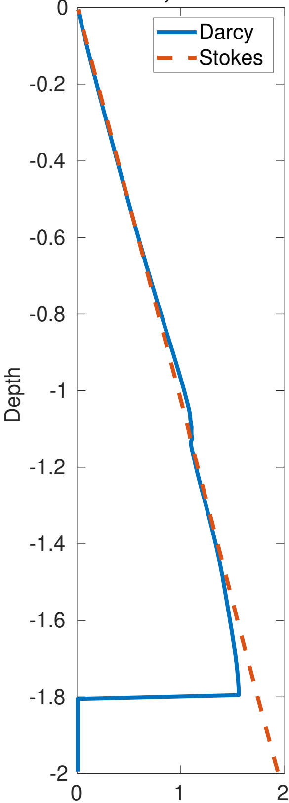
Pressure, t = 1000
