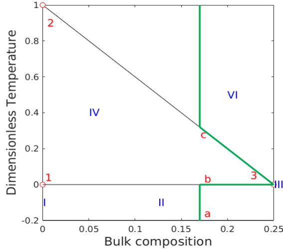
Figure 1.3: Phase diagram when the composition of opx is smaller than the eutectic composition. Region V does not appear.
