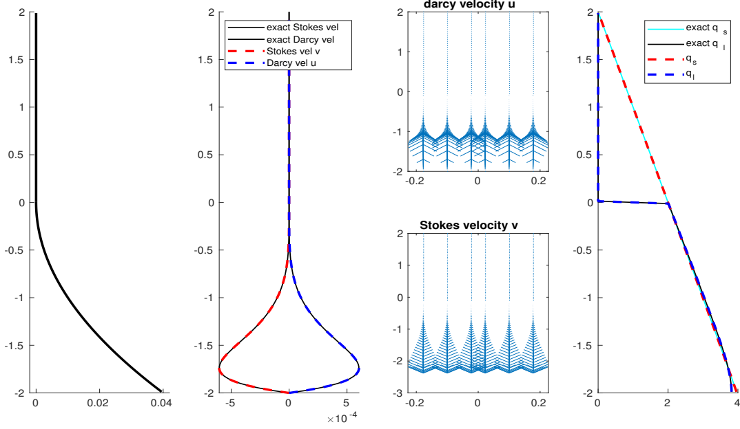
Figure 4: Quadratic porosity compaction column test \phi_0 = 0.01 .
