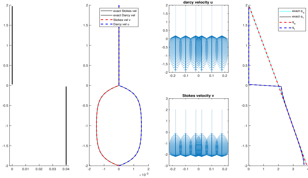
Figure 2.12: Discontinuous porosity (2.158) with \phi_0 = 0.04 . Shown are the porosity \phi , scalar velocities u and v along with closed form solution, velocity vectors \tilde{\mathbf{v}}_s and \phi\tilde{\mathbf{v}}_r reconstructed on the edge quadrature points, q_l and q_s together.
