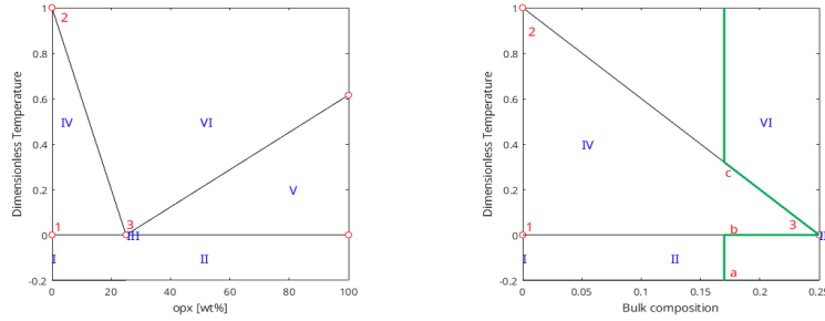
Figure 1.2: Eutectic Phase Diagram. 1) Full phase diagram of olivine-opx system. 2) Phase diagram when composition of opx smaller than eutectic composition.
