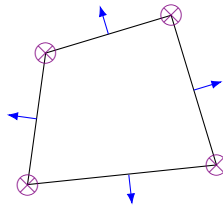
Figure 3.2: An exhibition of velocity dofs associated with a modified Bernardi-Raugel element.
