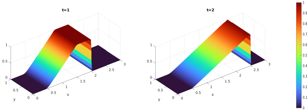
Figure 7: The reconstructed solution on the 180 \times 60 rectangular mesh at times 1.0 and 2.0. (The rarefaction and shock meet at time 2.0.)
