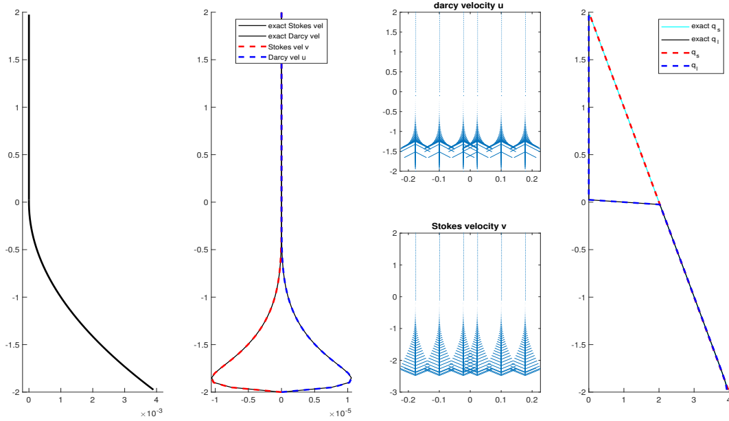
Figure 2.13: Quadratic porosity (2.159) with \phi_0 = 0.001 . Shown are the porosity \phi , scalar velocities u and v along with closed form solution, velocity vectors \tilde{\mathbf{v}}_s and \phi\tilde{\mathbf{v}}_r reconstructed on the edge quadrature points, q_l and q_s together.
