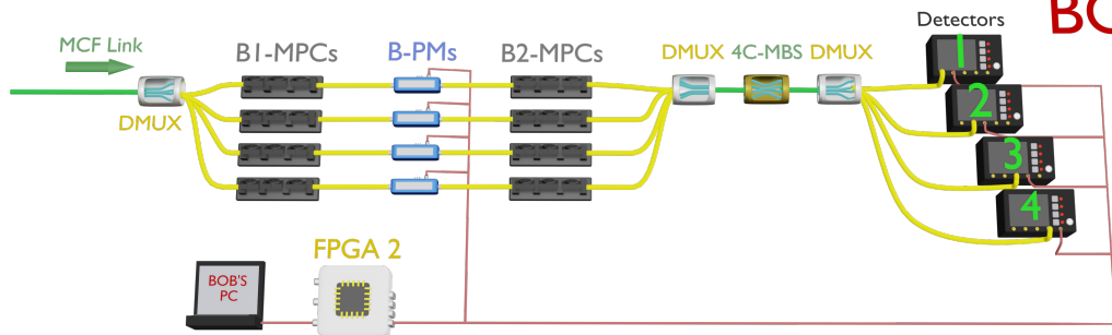
Figure 3.3.1: Experimental setup (Alice and Bob's stages). Yellow lines indicate SMFs. Green lines indicate 4C-MCFs. Red lines indicate electrical cables. Detectors are numbered from 1 to 4 in the figure for clarity, corresponding to detectors 0 through 3 in the text. FPGAs and detectors synchronized through separate cables (not shown for clarity).
