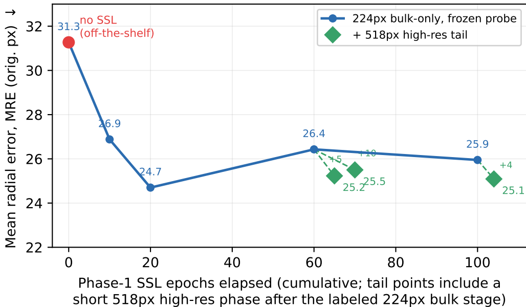
(a) 224px bulk-adaptation duration + high-res tail — fold-0 internal
