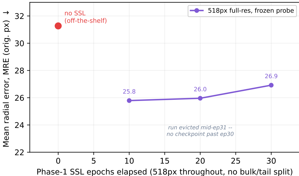
(b) 518px full-resolution control — fold-0 internal
