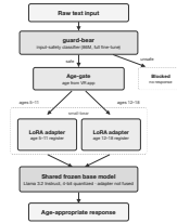
Fig. 1 System architecture. guard-bear (86M params, <50ms) screens input before an age-gate routes safe queries to one of two LoRA adapters on a shared frozen 4-bit Llama 3.2 base; adapters are never fused. Rank/layer and base size are runtime choices behind each adapter box, not drawn separately – Table 1’s four configurations are all instances of this diagram.
